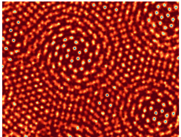
Above: Molybdenum disulfide.
